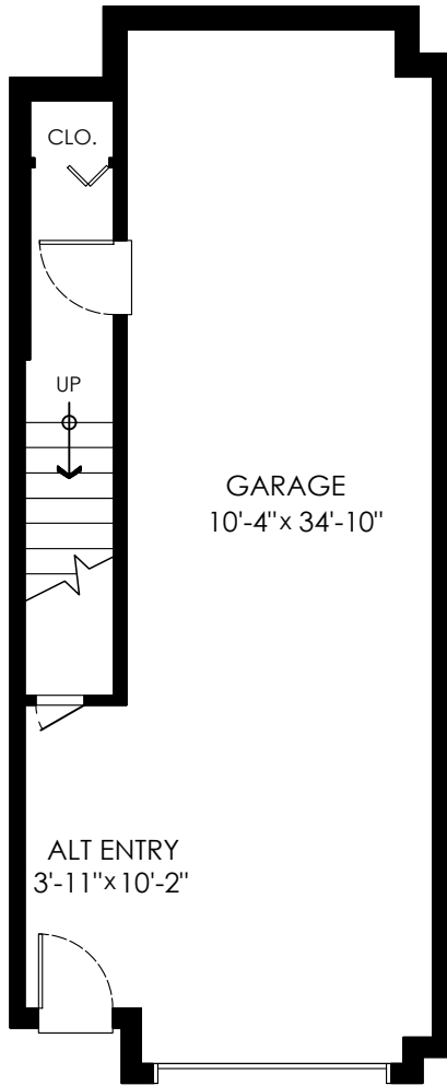
Lower Floor Plan Floor Area: 83 sq.ft. Ceiling Height: 8'-3"
