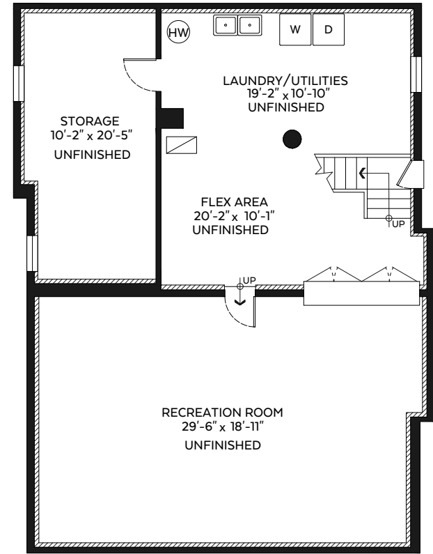
Lower Floor Plan Unfin. Floor Area: 1,310 sq.ft.
