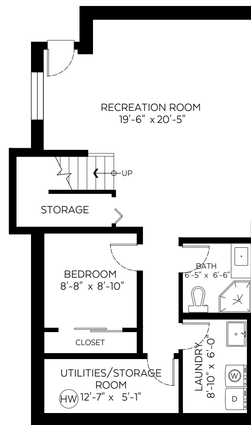
Lower Floor Plan Floor Area: 830 sq.ft. Ceiling Height: 8.75 ft.
