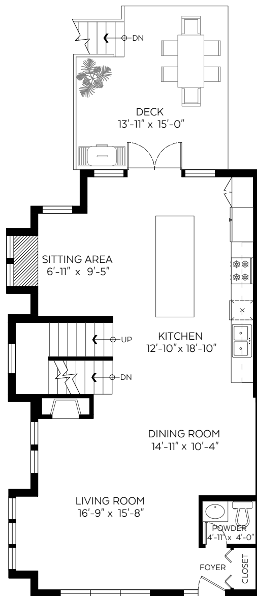
Main Floor Plan Floor Area: 847 sq.ft. Ceiling Height: 8.75 ft.
