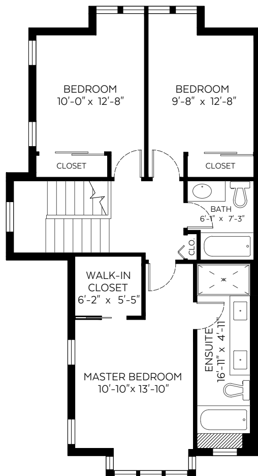
Upper Floor Plan Floor Area: 819 sq.ft. Ceiling Height: 8 ft.
