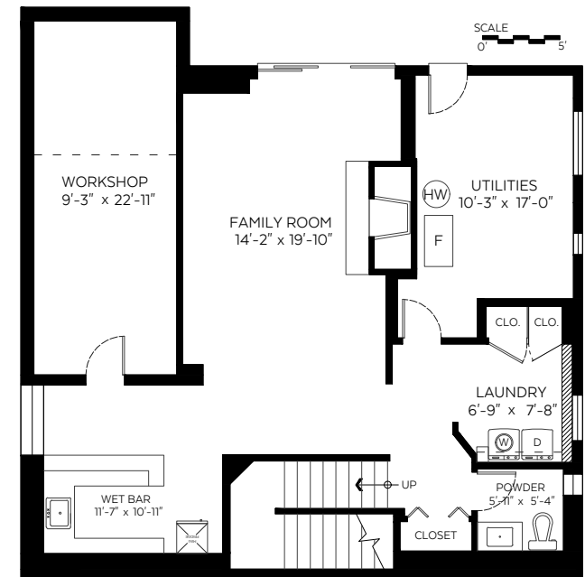
Lower Floor Plan Floor Area: 1,251 sq.ft.
