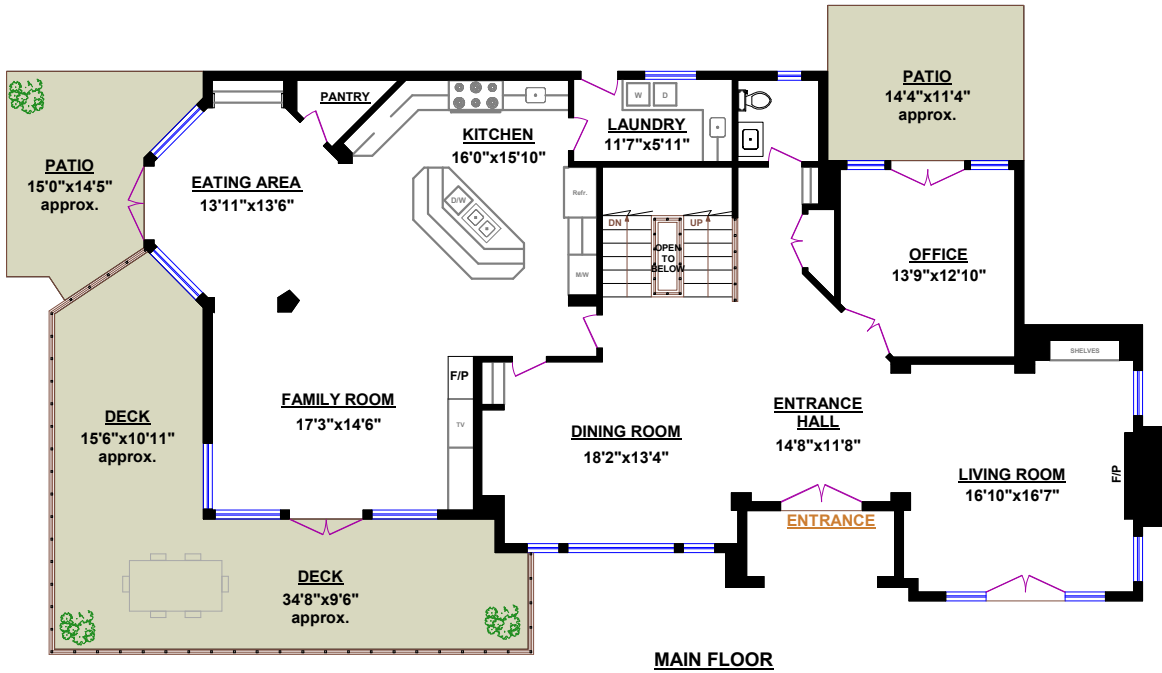
MAIN FLOOR
