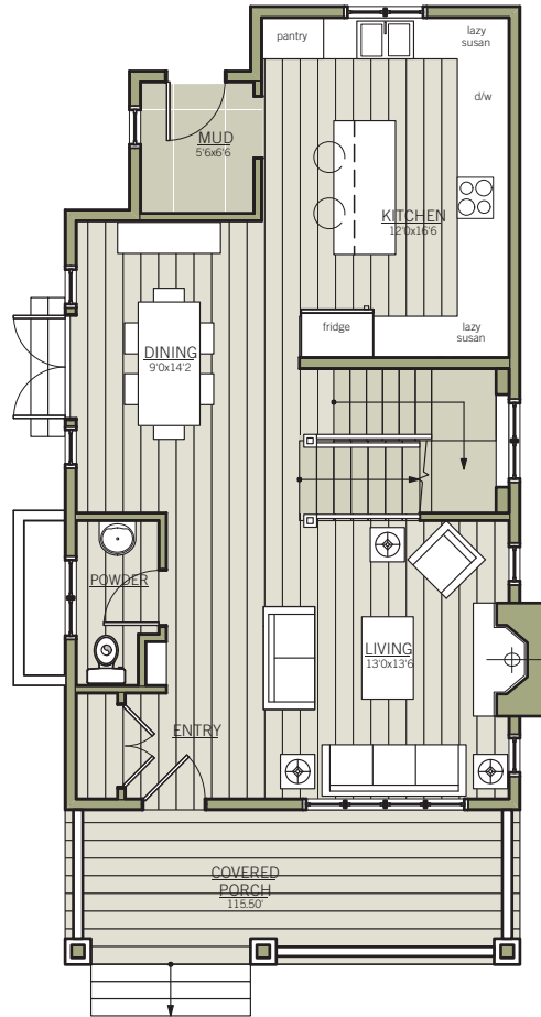
MAIN FLOOR PLAN 820 SQ FT APPROX
