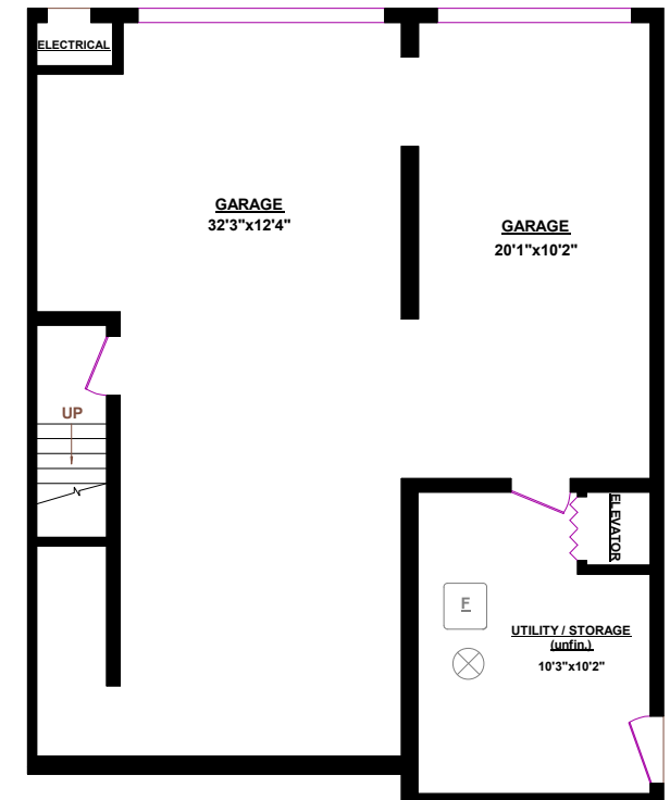
BASEMENT
