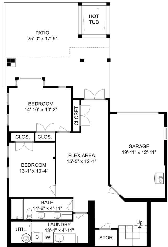
LOWER FLOOR 1,020 sq.ft. | Ceiling Height: 8'-0"
