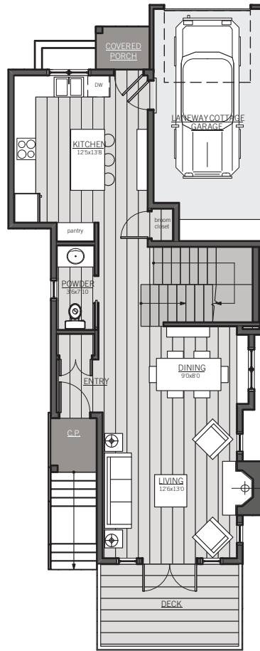
MAIN FLOOR PLAN 720 SQ FT APPROX
