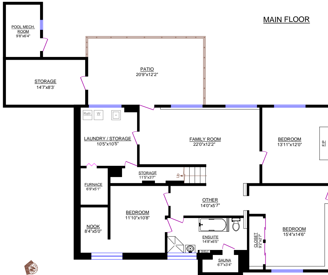
LOWER LEVEL
